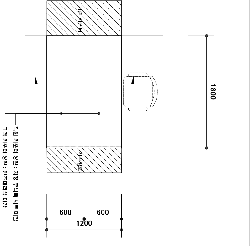
1 카운터(TOP VIEW) SCALE A1 1/20 A3 1/40
